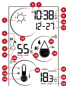
Illustration 2: Parts overview for base station
